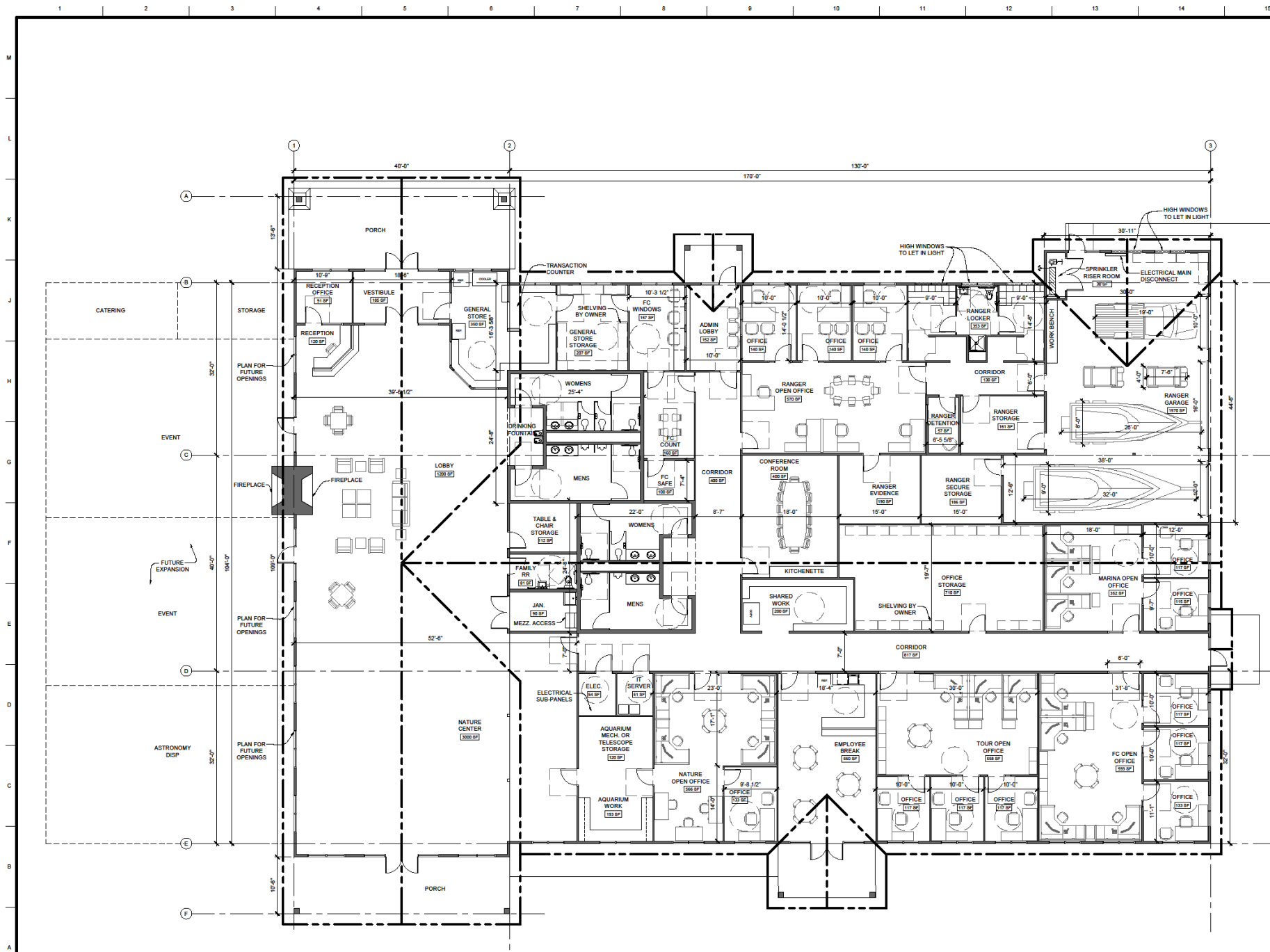
FLOOR PLAN- 17,430 SQ FT
